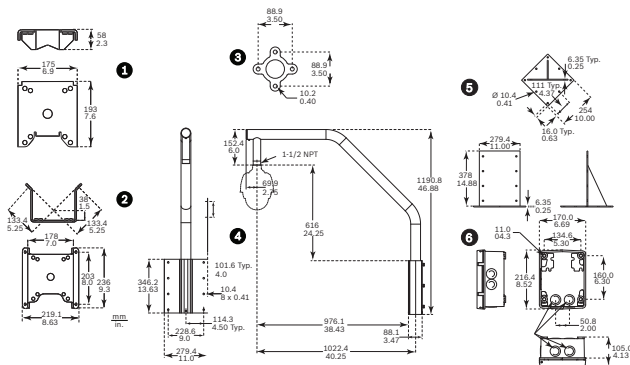
AUTODOME 7000 Series, optionele montagebeugels
