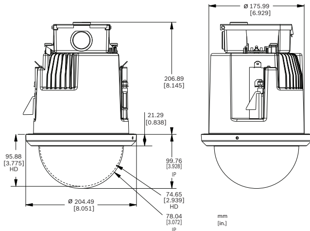
AUTODOME 7000 Series, plafondmontage
