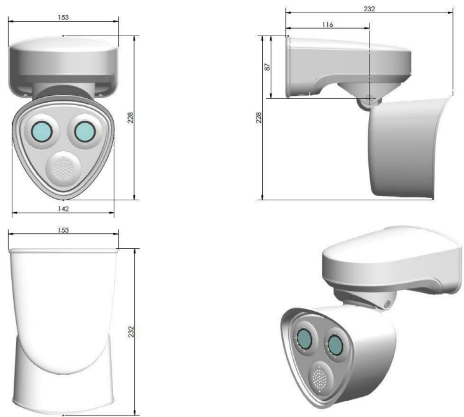
Fig. 1: MOBOTIX M73 EN54: All measurements in mm
