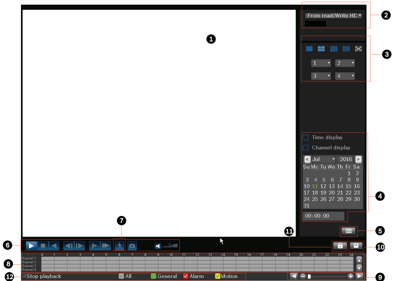
Figure 9.4: Search/Play screen
