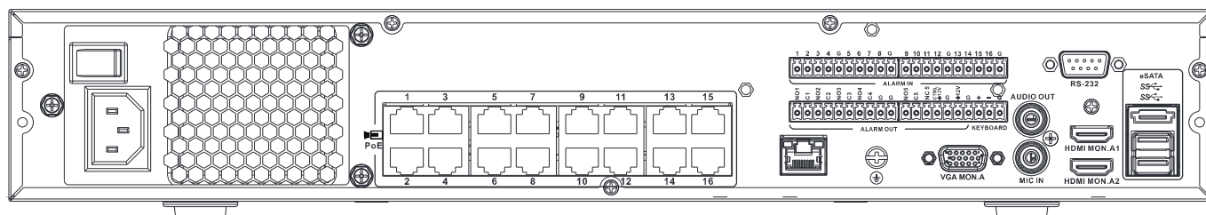
Achterpaneel DIVAR 5000 network (16 PoE)
