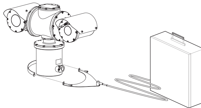
<Standard method to install camera and washer pump>
